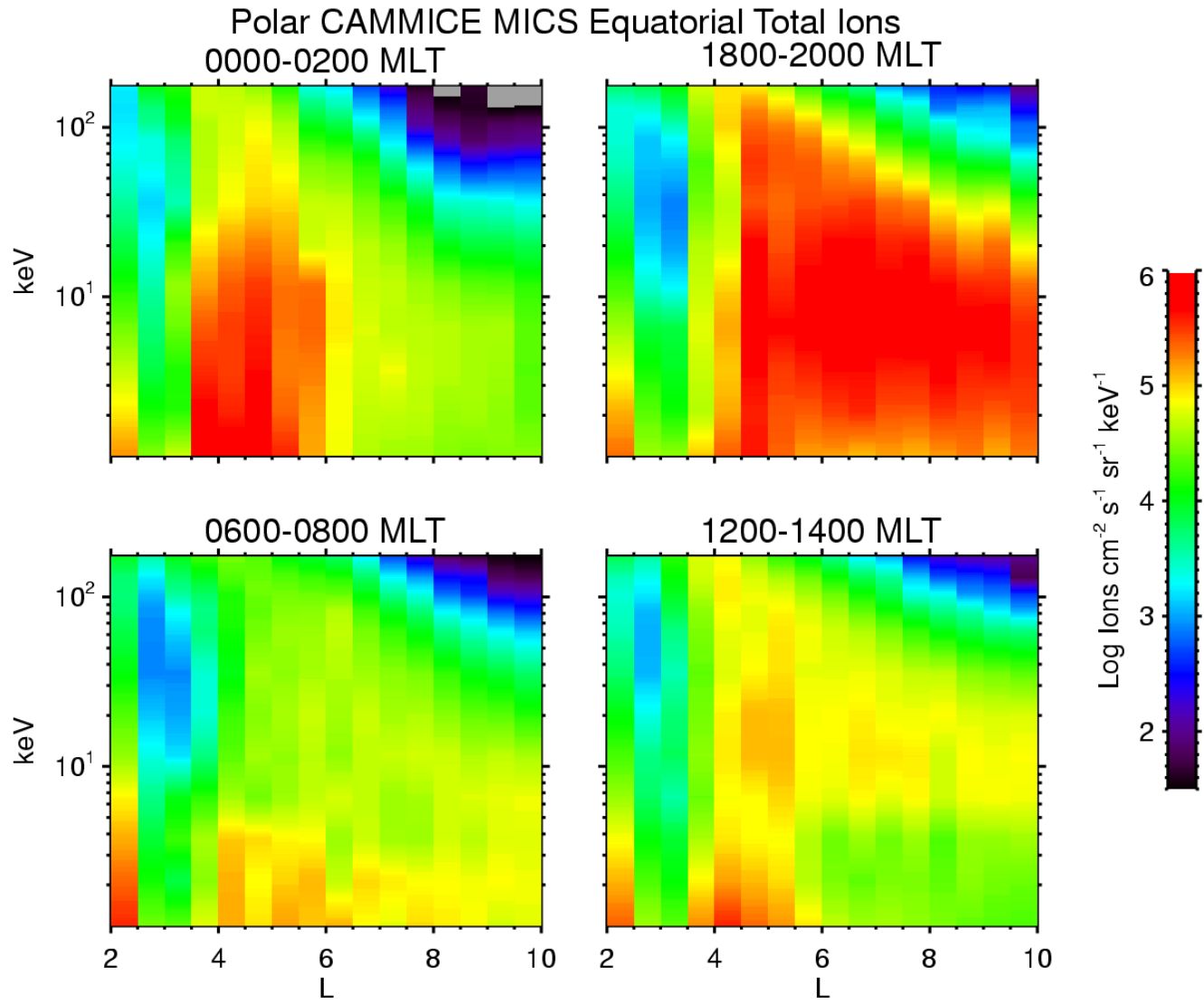
Data Interval: Feb 1996 - Sept 1999 All Geomagnetic Activity Levels Included
